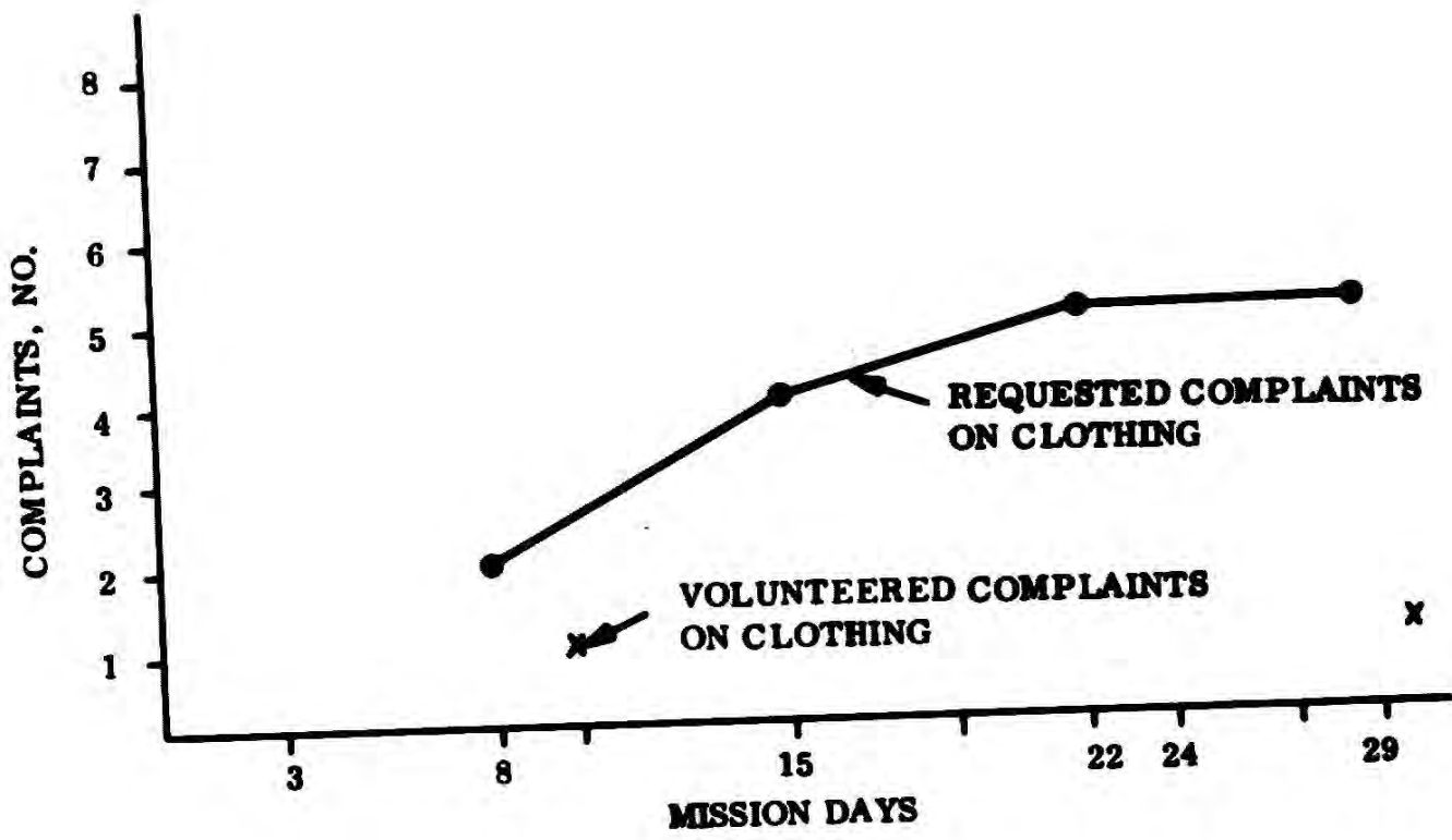
Figure 6-1. Clothing Complaints
