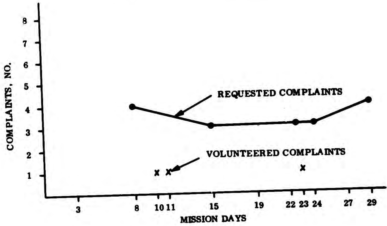
Figure 6-2. Bedding Complaints
