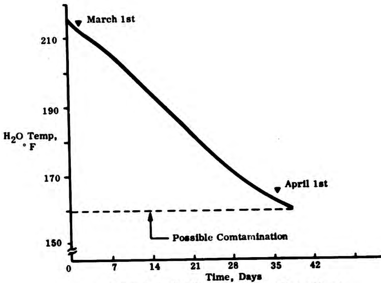
Figure 5-2. Hot Water Tank Temp Decay Curve
