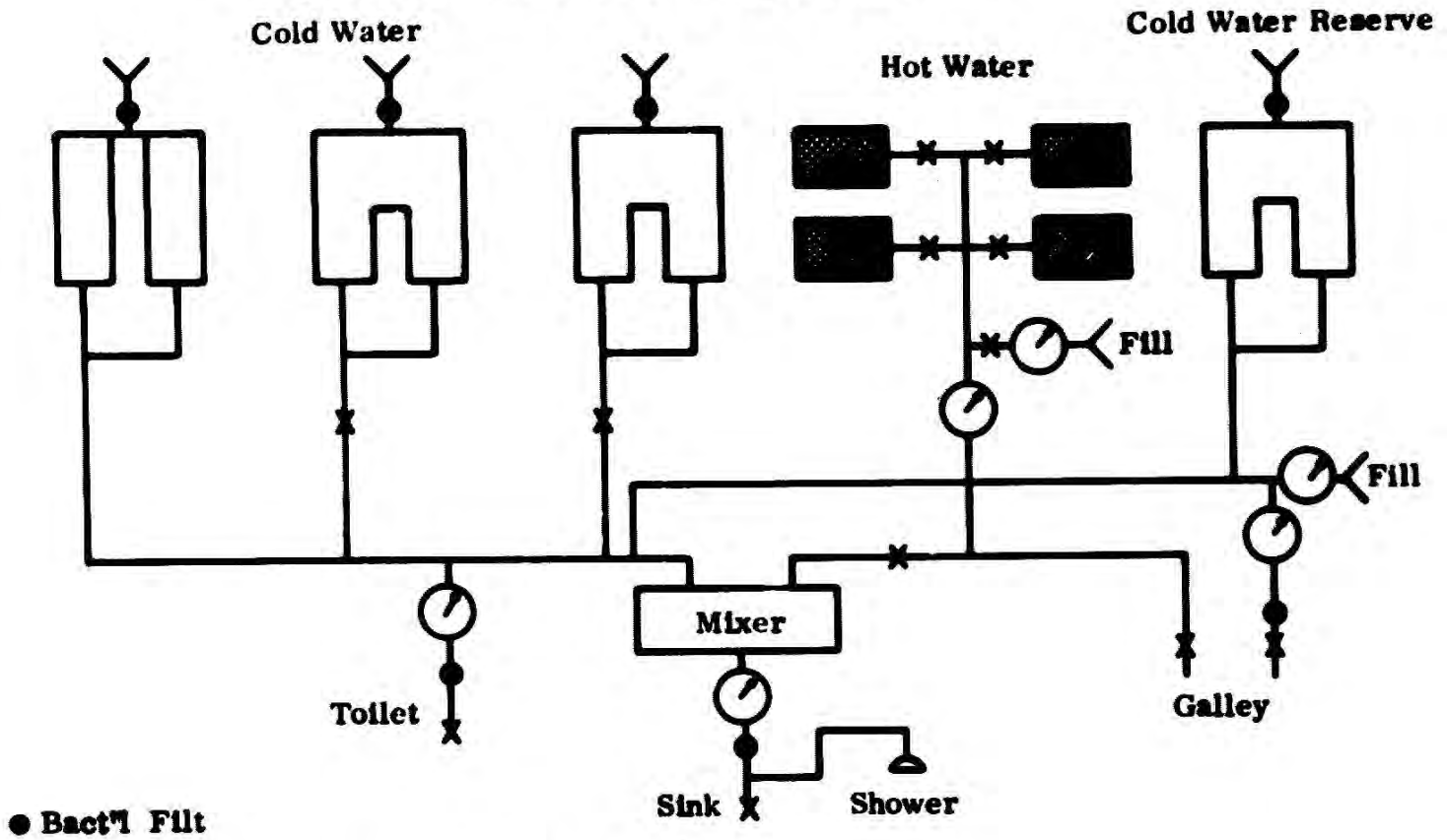
Figure 5-3. Water Management System
